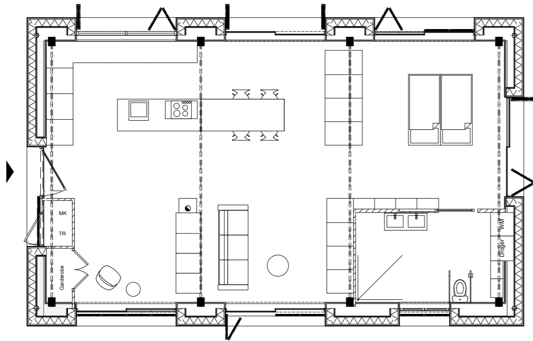
Begane grond | Ground floor
